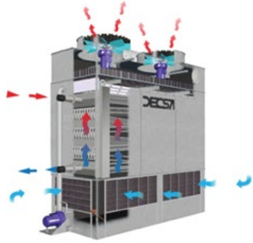
KAPALI TİP AKSİYEL FANLI KULE REFA - CFR-A
